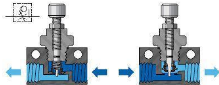
Figure 2: Conventional Flow Regulators
