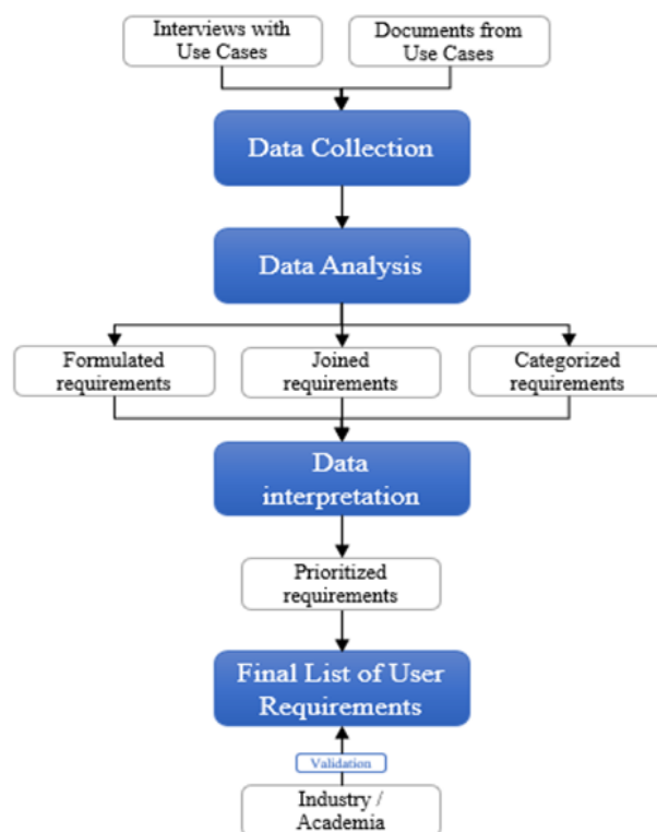
Figure 1. The process of formulating URs in CoLLaboratE
