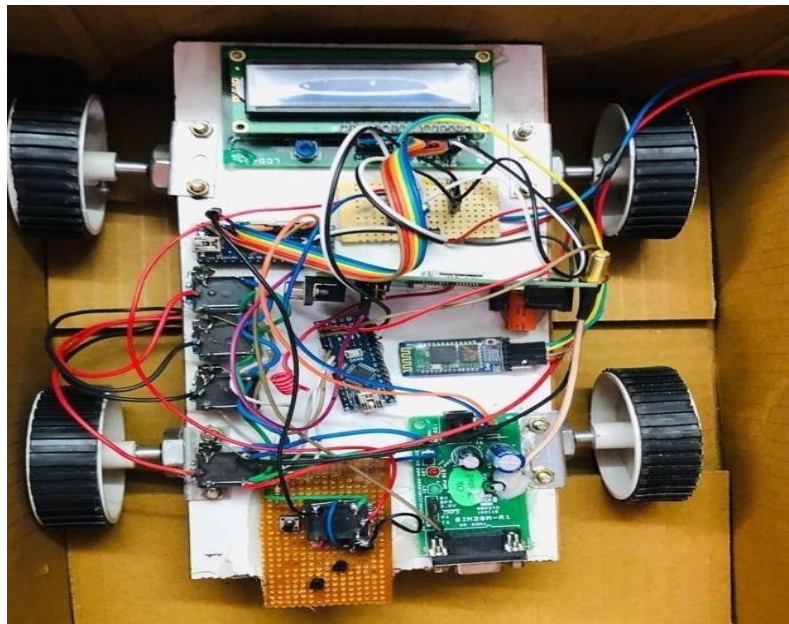
Fig. No.: 1 Prototype of the robot
