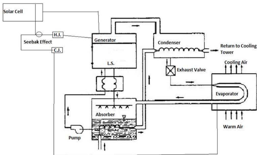
Fig.1: Schematic diagram of LiBr/water based adsorption refrigerator
