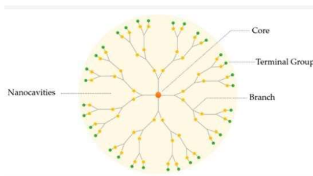
Figure: 3 Dendrimers
