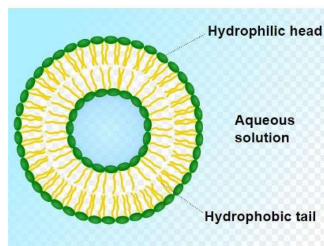
Figure: 1 Liposome
