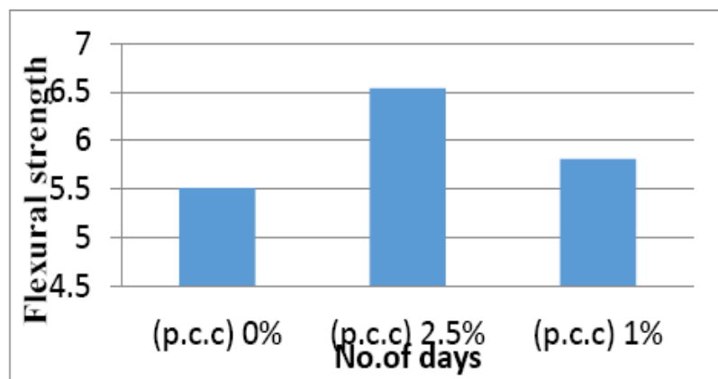
Fig 12 Flexural strength at 28 days
