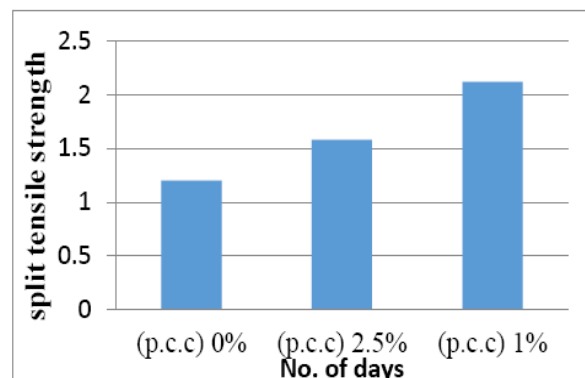
Fig 9 Split tensile strength at 7 days
