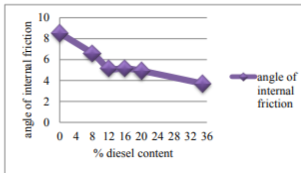
Fig. 9 Angle of Internal friction of Contaminated Clay
