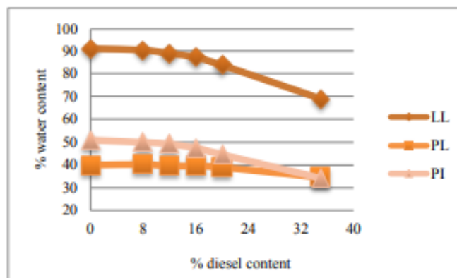
Fig. 10 Atterberg Limits of Contaminated Clay
