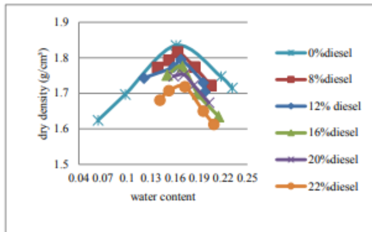
Fig. 5 OMC and MDD of contaminated lateritic soil
