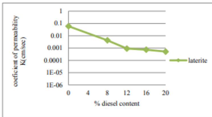
Fig. 4 Permeability of contaminated Lateritic soil
