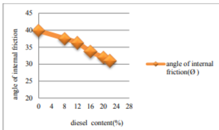
Figure . 1. Angle of internal friction of contaminated lateritic soil
