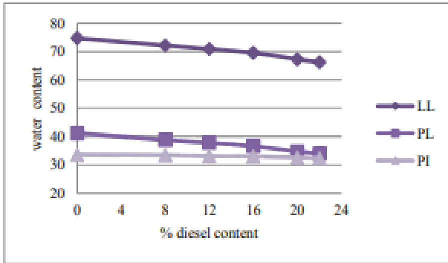
Fig. 3 Atterberg limits of Contaminated Lateritic soil
