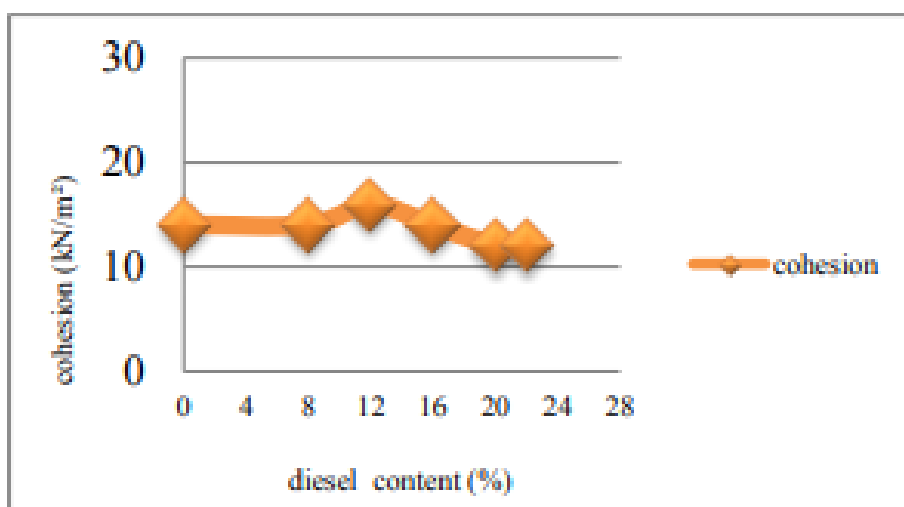
Fig. 2 Cohesion of contaminated lateritic soil
