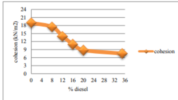
Fig 8 Cohesion Values of Contaminated Clay
