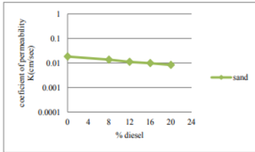
Fig. 7 Permeability of Contaminated Sand
