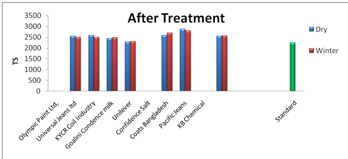
Figure 4: Comparison of TS of different industries after treatment.
