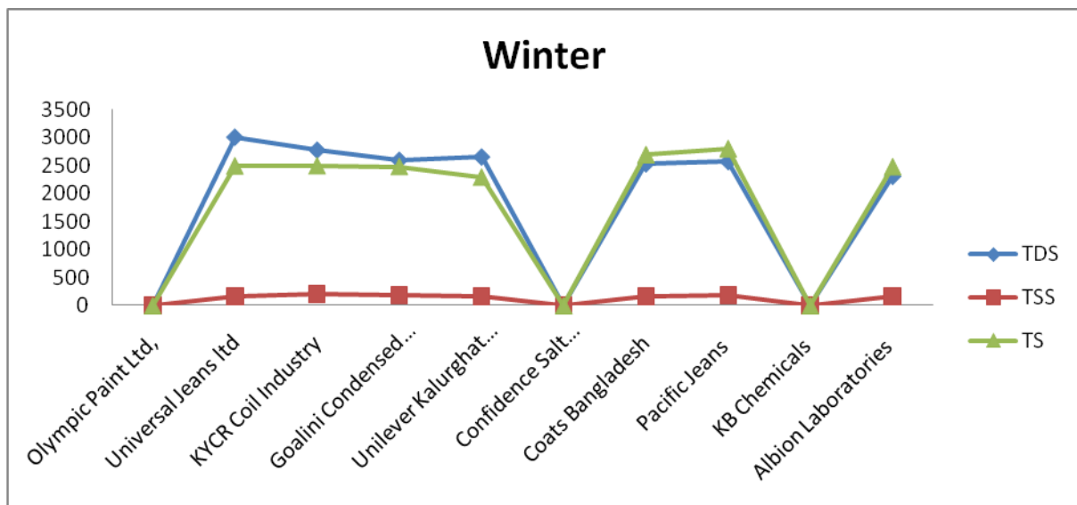
Figure 6: Comparative measurement of TDS, TSS and TS in winter season, after treatment
