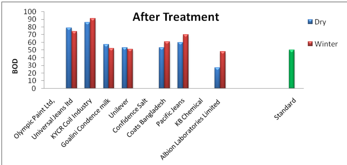
Figure:-10 Comparison of BOD of different industries after treatment.
