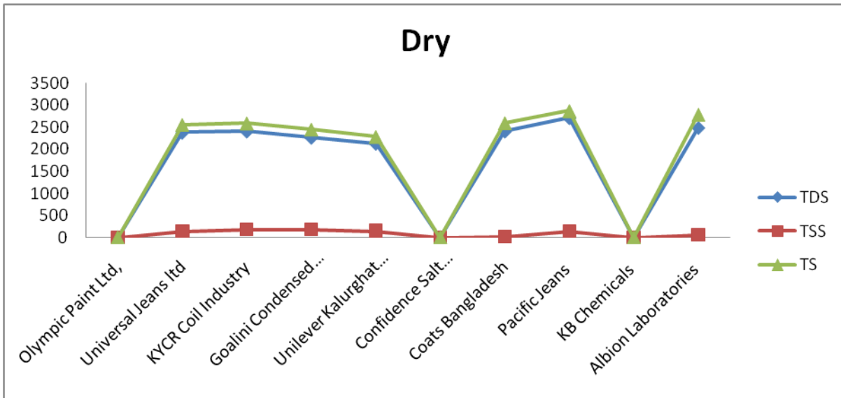
Figure 5: Comparative measurement of TDS, TSS and TS in dry season, after treatment
