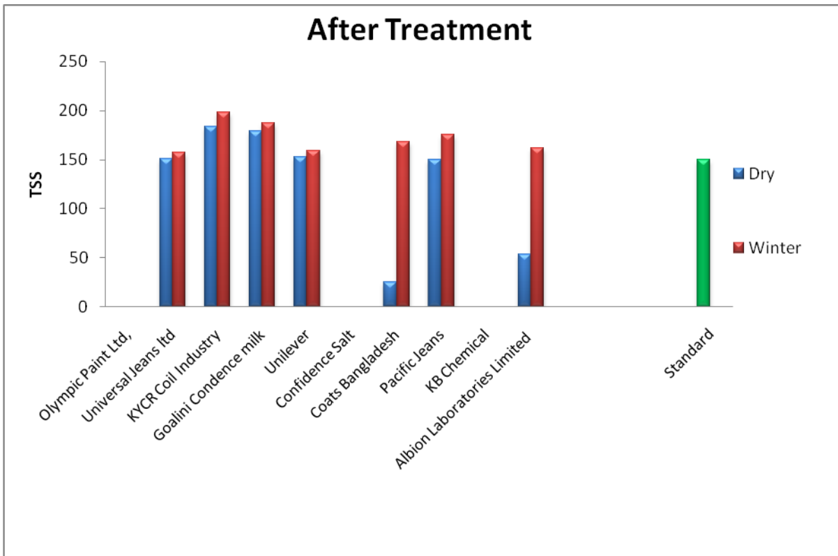
Figure 2: Comparison of TSS of different industries after treatment.
