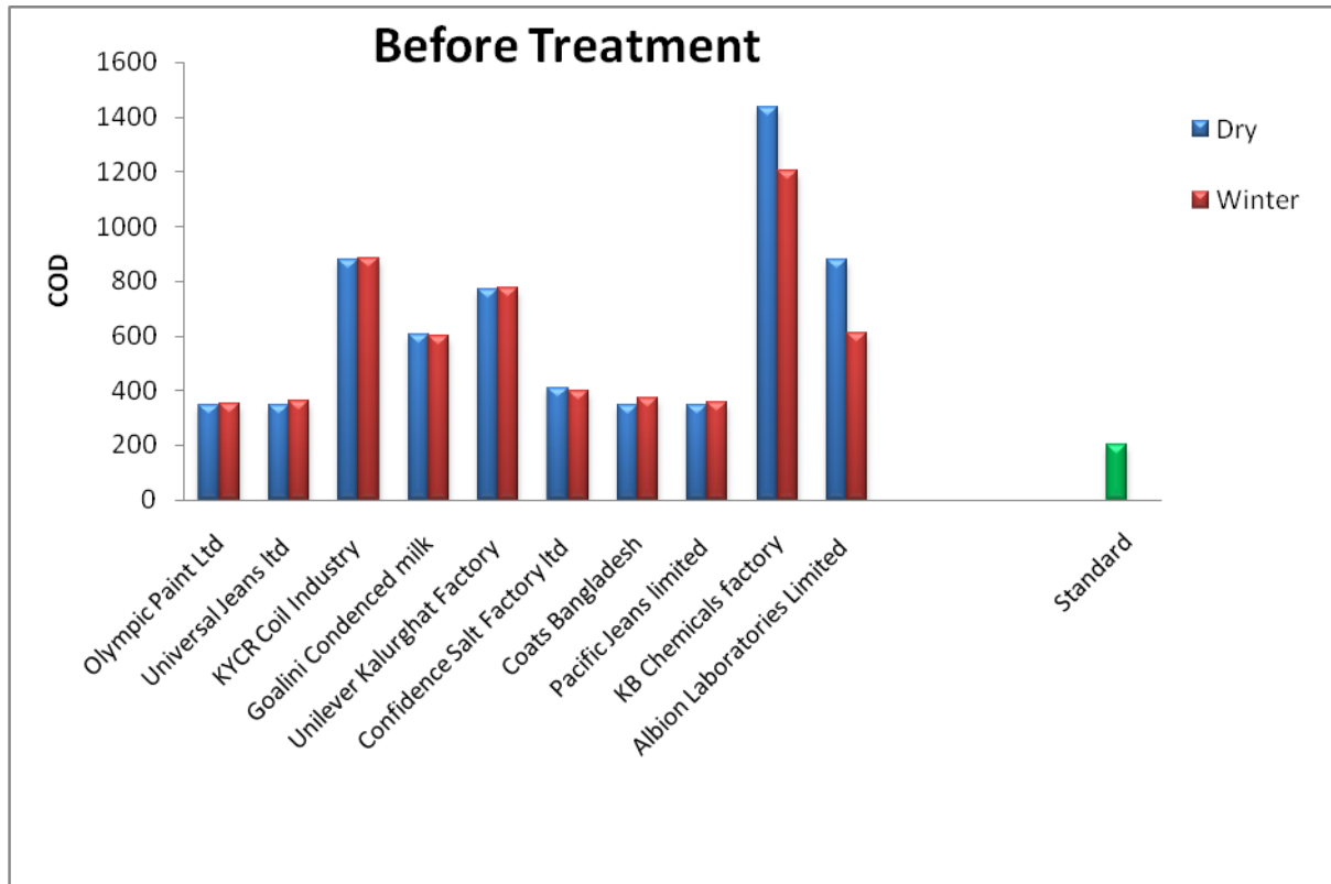
Figure:-11 Comparison of COD of different industries before treatment.
