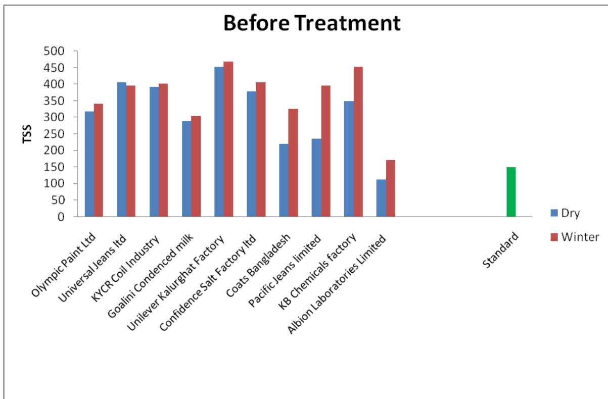
Figure 1: Comparison of TSS of different industries before treatment
