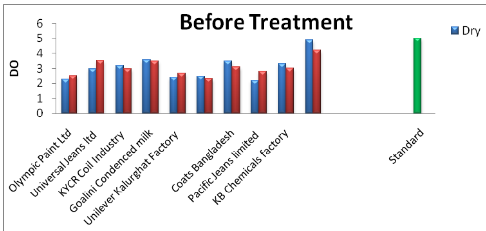
Figure 7: Comparison of DO of different industries before treatment.
