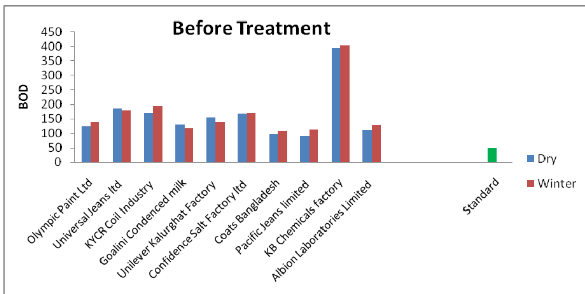
Figure:-9 Comparison of BOD of different industries before treatment.
