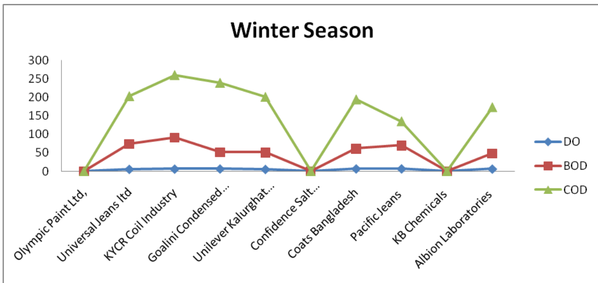
Figure:-14 Comparative measurement of COD, BOD and DO in winter season, after treatment
