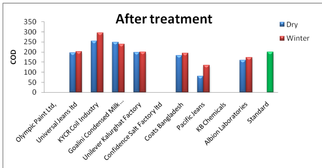
Figure:-12 Comparison of COD of different industries after treatment.
