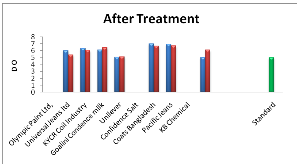
Figure 8: Comparison of DO of different industries after treatment.
