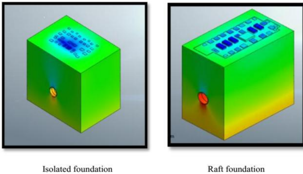
Figure no:-2 Size of models and loading on foundations
