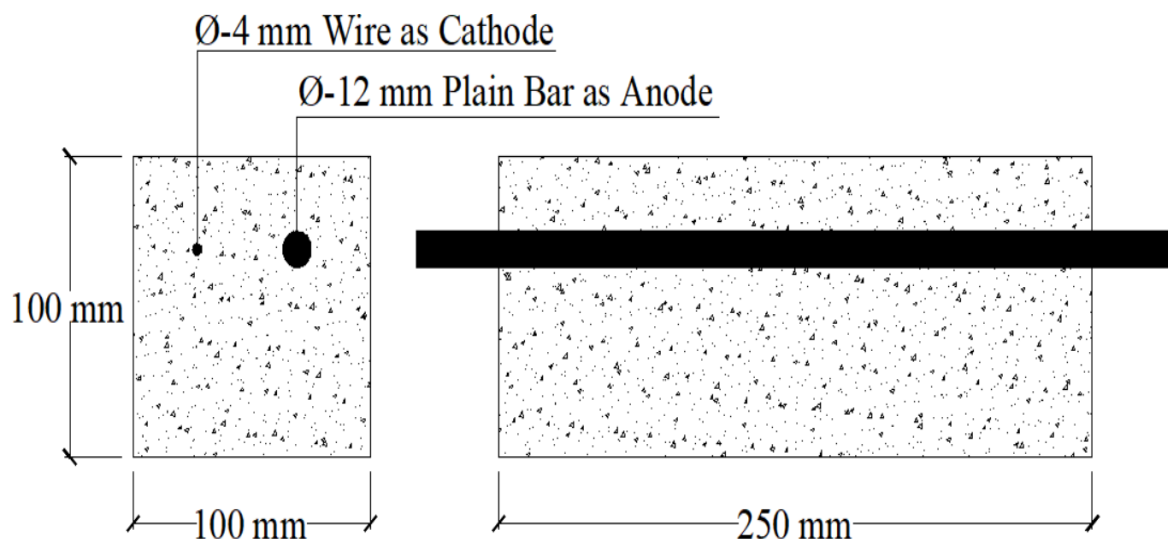
Figure 1: Schematic Diagram of Test Specimen
