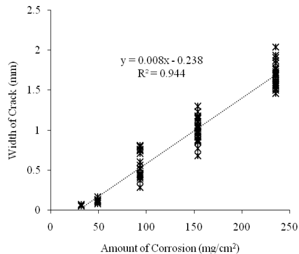
Figure 3: Variation of Crack Width with the Level of Corrosion
