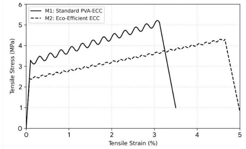
Figure 1: Stress-Strain Relationship for ECC Mixes under Uniaxial Tensile Loading
