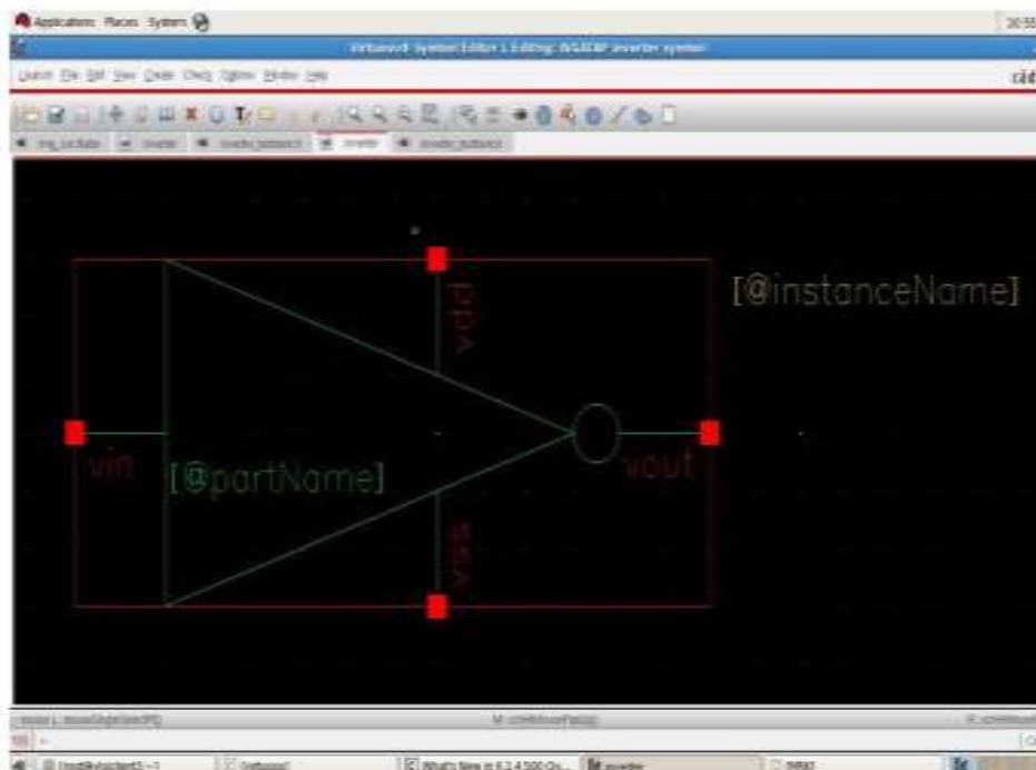
Figure 4.2 Symbol of an Inverter
