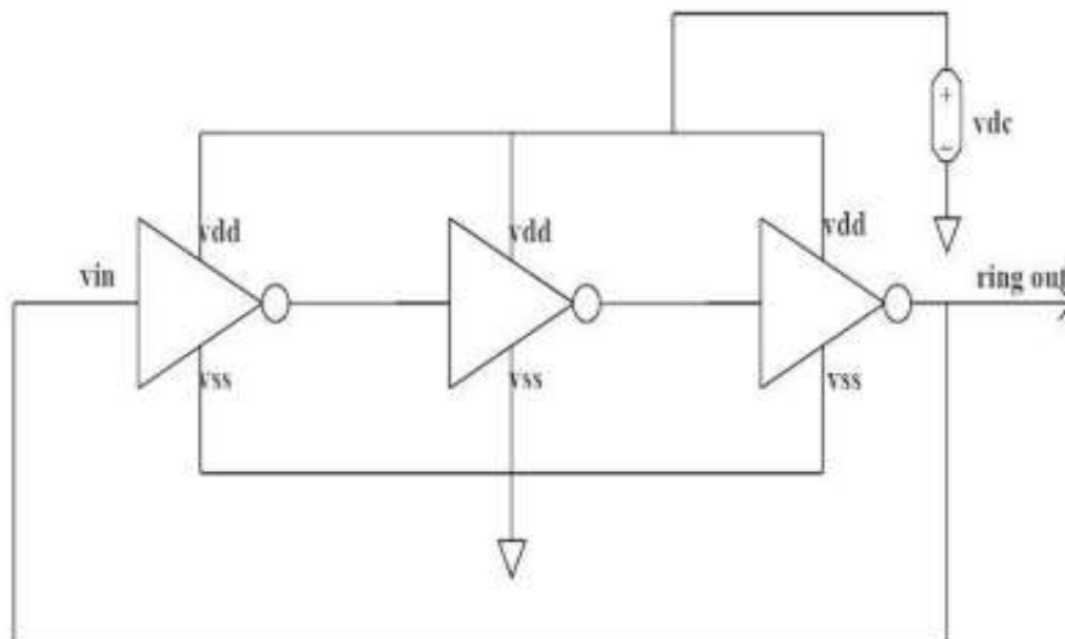
Figure 3 Schematic of Ring Oscillator
