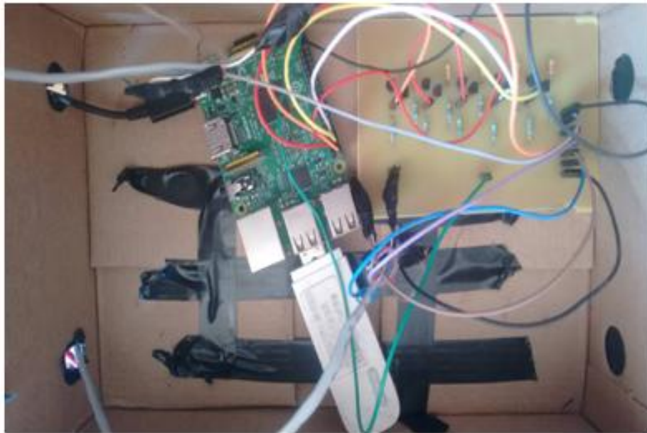
Fig. 4 '3G' dongle connected to raspberry pi
