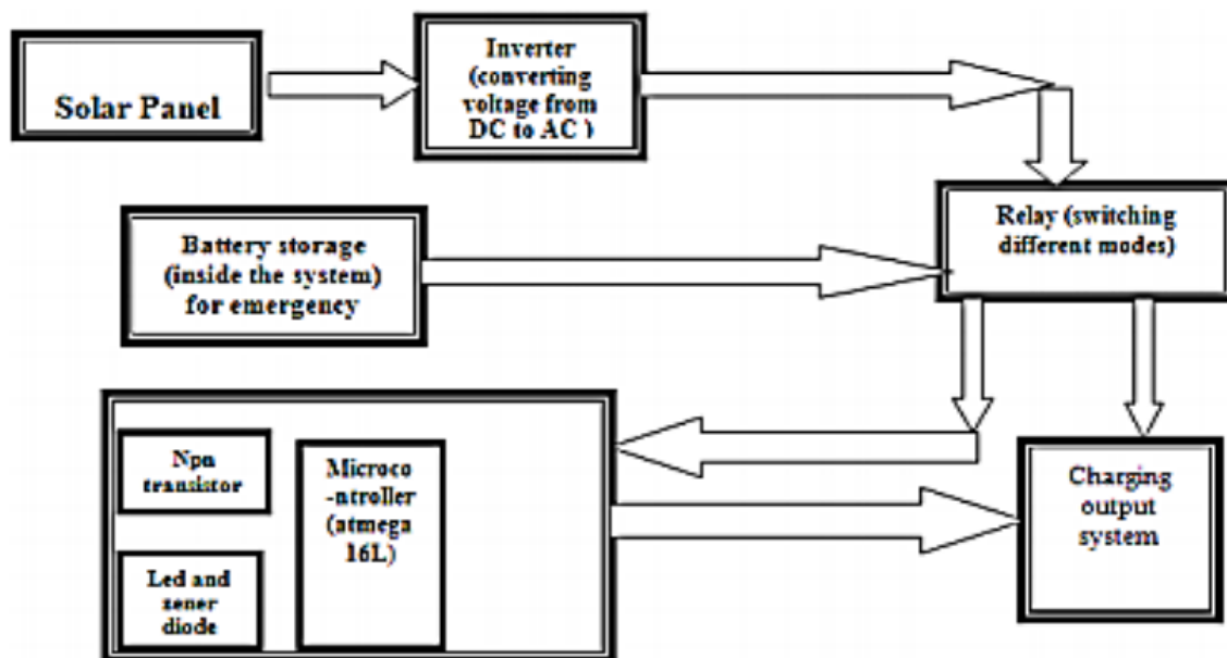
Fig: 2. Proposed system block diagram
