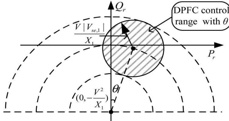
Fig. 5: DPFC active and reactive power control range with the transmission angle \theta .
