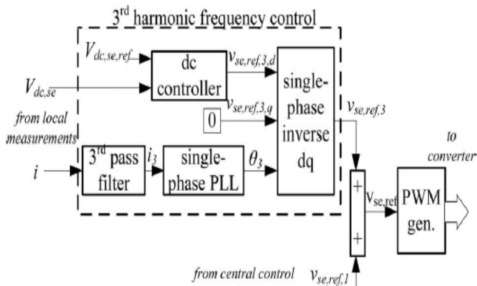
Fig. 7: Block diagram of the series converter control.
