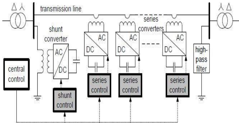
Fig. 6: DPFC control block diagram.
