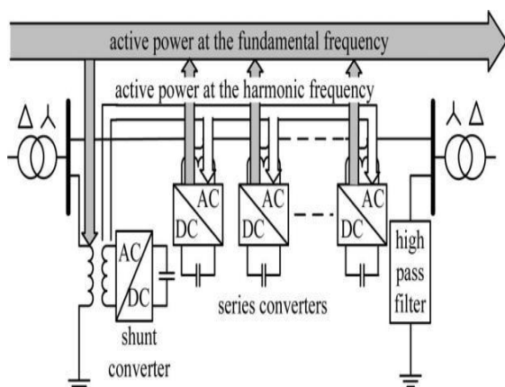
Fig. 3: DPFC configuration.
