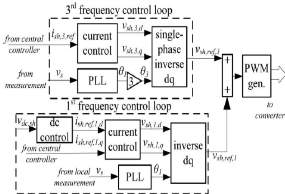
Fig. 8: Block diagram of the shunt converter control
