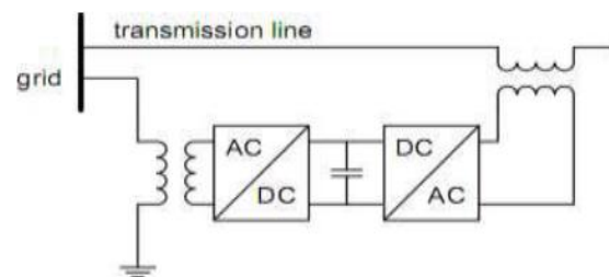
Fig.1: Simplified representation of a UPFC
