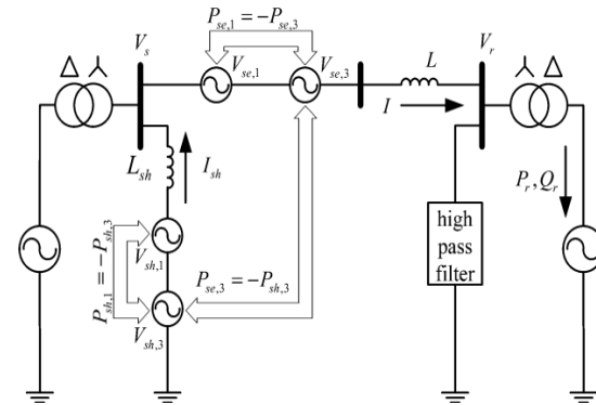
Fig. 4: DPFC simplified representation
