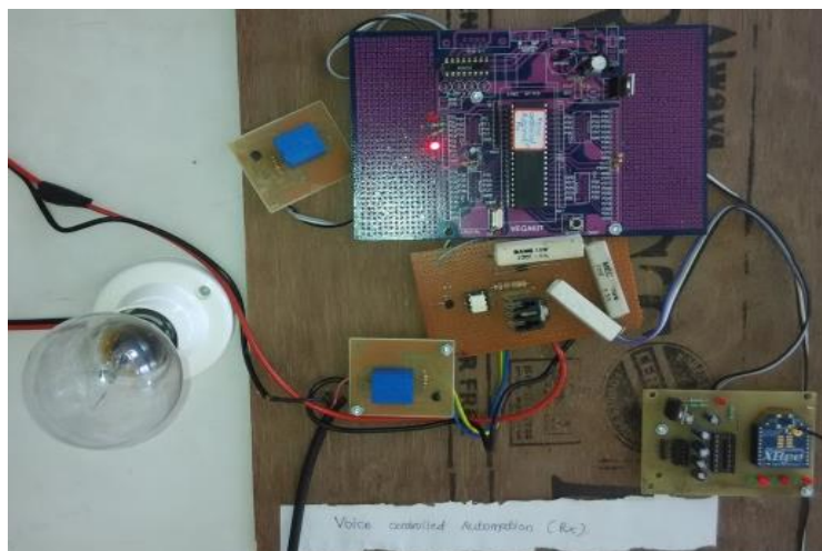
Figure 5: Receiver section
