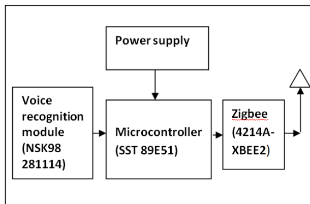
Figure 2: Transmitter
