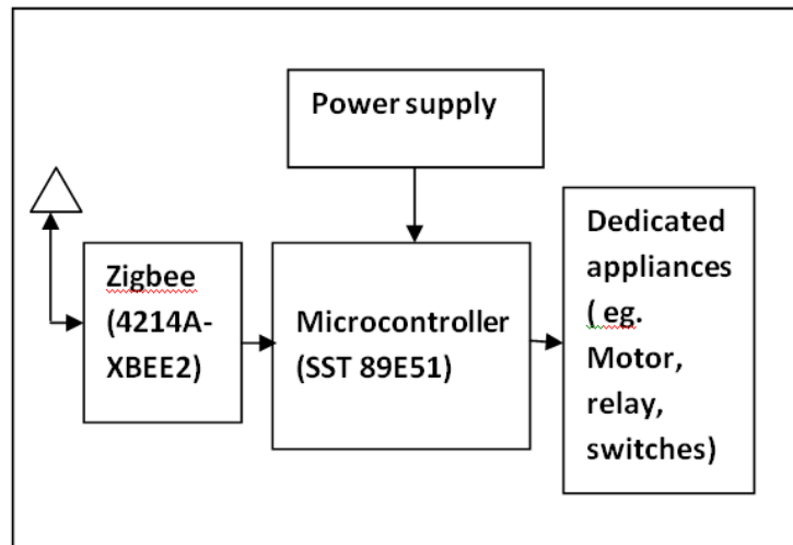
Figure 3: Receiver
