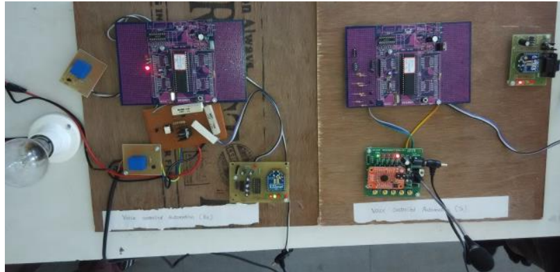
Figure 6: “Speech Authenticated Automatic Industry Sway” system
