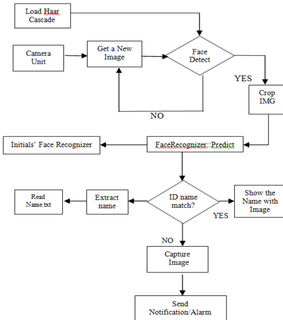
Fig.6:Face Recognition Flow chart
