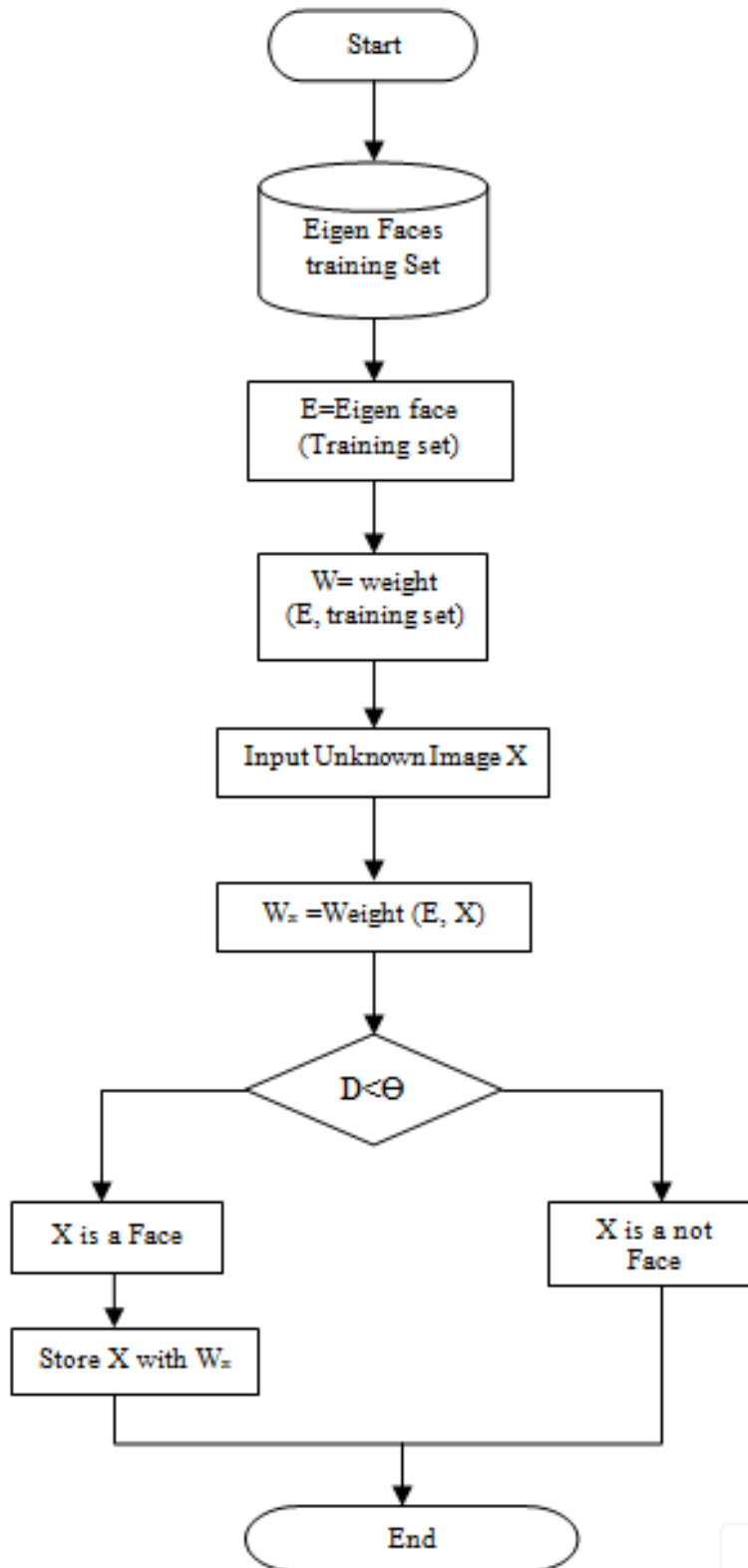
Figure 3: High-level functioning principle of the Eigenface-based facial recognition algorithm
