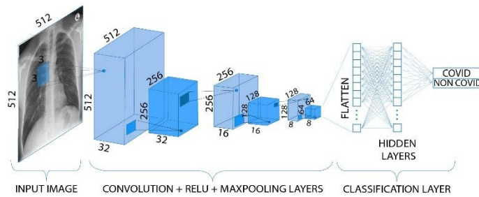
Fig. 3: Deep Learning Network used in the model
